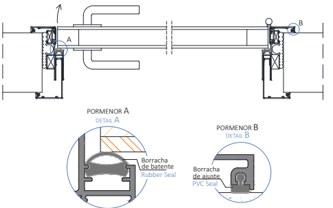
SIMPLES ABRIR SINGLE DOOR
