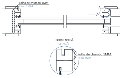
SIMPLES CORRER SINGLE SLIDING DOOR
