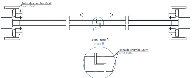
DUPLO CORRER DOUBLE SLIDING DOOR
