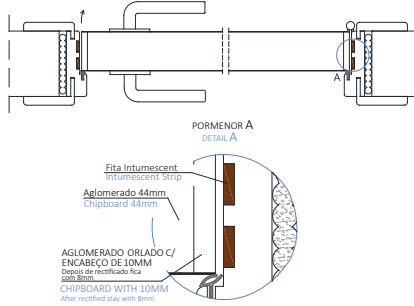
SIMPLES ABRIR SINGLE DOOR
