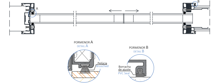
DUPLO CORRER DOUBLE SLIDING DOOR
