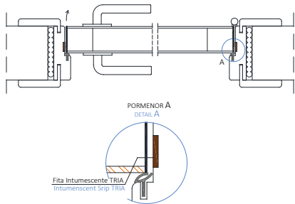
SIMPLES ABRIR SINGLE DOOR
