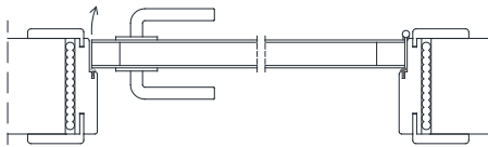
SIMPLES CORRER SINGLE SLIDING DOOR
