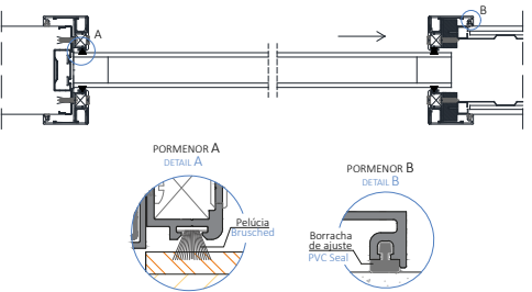
SIMPLES CORRER SINGLE SLIDING DOOR
